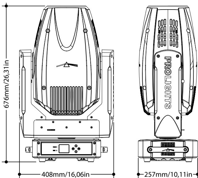
Technical drawing
