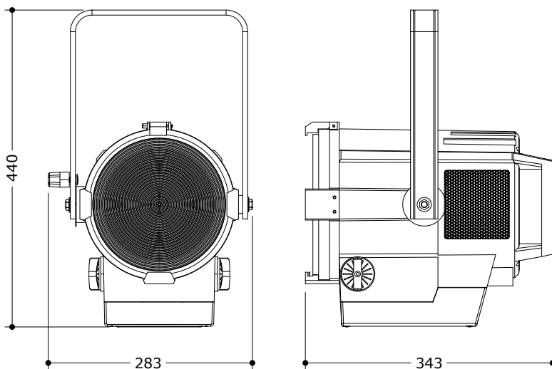
Technical drawing
