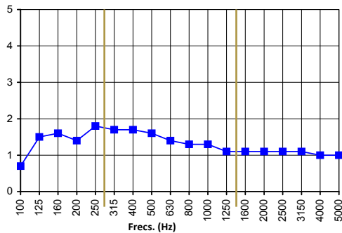
Object's equivalent sound absorption area, A obj (m²)
