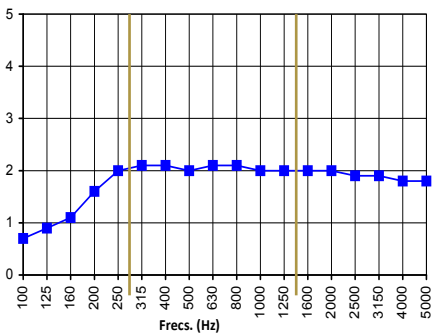
Object's equivalent sound absorption area, A obj (m²)
