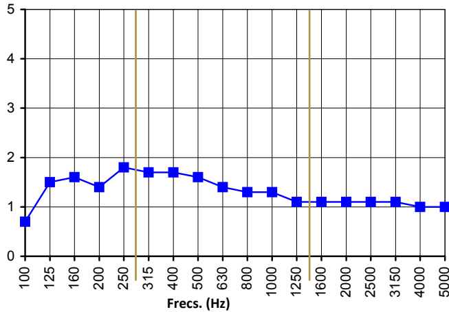
Object´s equivalent sound absorption area, Aobj (m²)
